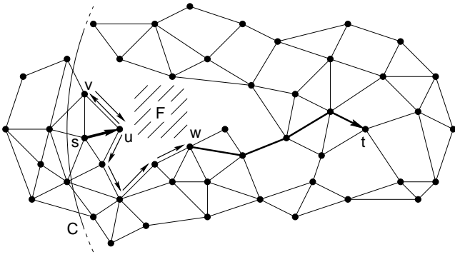
Figure 1: The GOAFR + algorithm starts from s in greedy mode. At node u it reaches a local minimum, a node without any neighbors closer to t . GOAFR + switches to face routing mode and begins to explore the boundary of face F (in clockwise direction). At node v the algorithm hits the bounding circle C and turns back to continue the exploration of F 's boundary in the opposite direction. After each step the counters p and q are updated. At node w the fallback condition p > \sigma q holds ( p = 2, q = 4 with the assumption 1/4 \leq \sigma < 1/2 ); GOAFR + falls back to greedy mode and continues to finally reach t . (Gradual reduction of C 's size during GOAFR + 's execution is not shown.)
