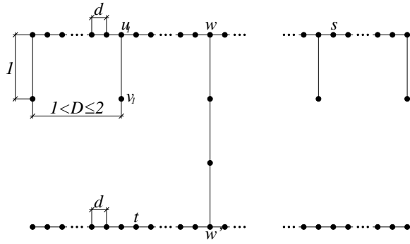
Figure 4: Lower bound graph for super-linear cost functions
