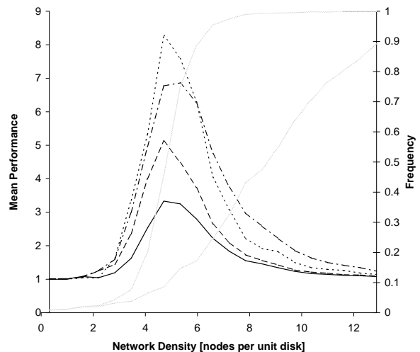
Figure 3: Performance of routing algorithms in critical network density range around 4.5 nodes per unit disk. Mean performance values for GOAFR + (solid line), GOAFR FC (dashed), GOAFR (dash-dotted), and GPSR (dotted) plotted against the left y axis. The network connectivity and greedy success rate are plotted for reference (in gray against right y axis).
