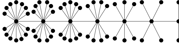
Figure 7.1: Distributed greedy algorithm: Bad example
