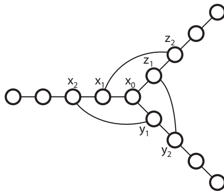
Figure 9.3: Counter example.
