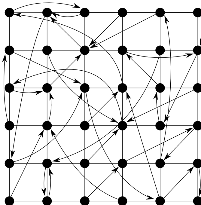
Figure 9.2: Augmented grid with m = 6
