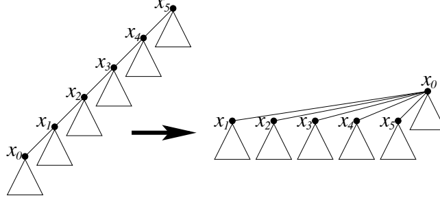
Figure 5.1: Reversal of the path x_0, x_1, x_2, x_3, x_4, x_5 .
