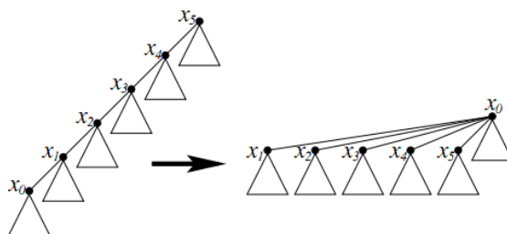
Figure 4.1: Reversal of the path x_0, x_1, x_2, x_3, x_4, x_5 .
