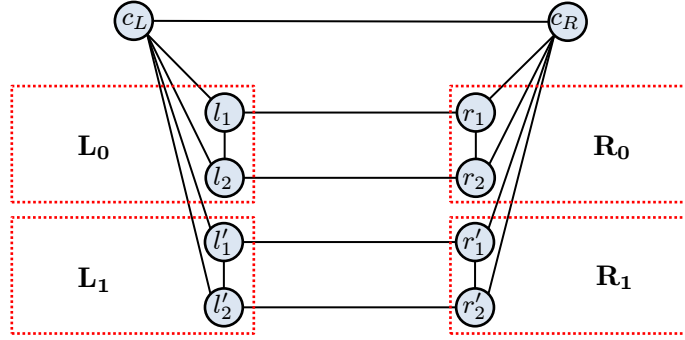
Figure 8.1: The above skeleton G' contains n = 10 nodes, such that q = 2 .
