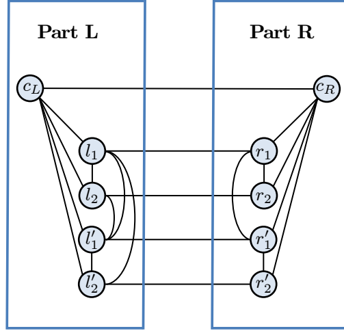
Figure 8.2: The above graph G has n = 10 and is a member of family \mathcal{G} . What is the diameter of G ?
