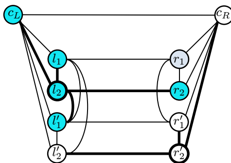
Figure 8.3: Nodes in the neighborhood of l_2 are cyan, the neighborhood of r'_2 is white. Since these neighborhoods do not intersect, the distance of these two nodes is d(l_2, r'_2) > 2 . If e.g. edge (l_2, l'_2) was included, their distance was 2.
