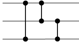
Figure 3: A correct sorting network that does not sort correctly when fed backwards.
